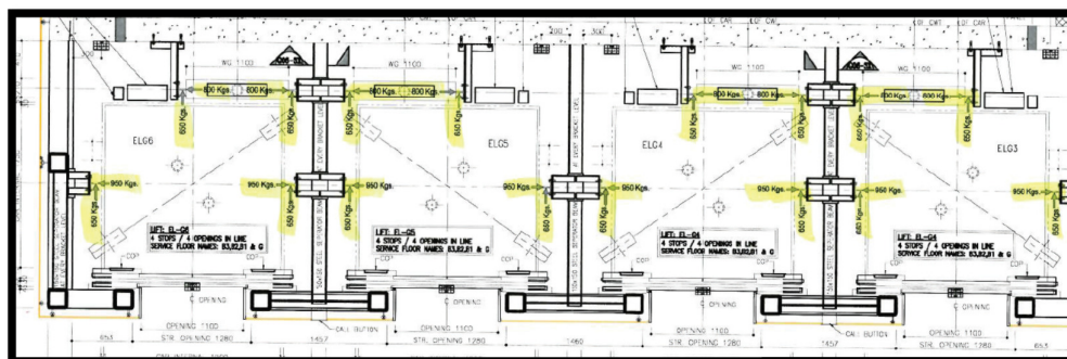
Shaft Plan with Rail Forces
